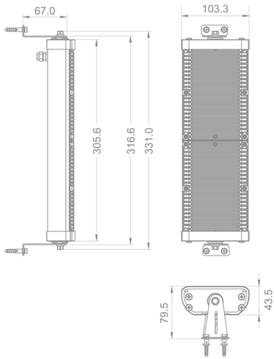
Solar Light
