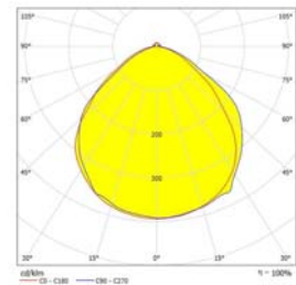
Luminance Distribution
