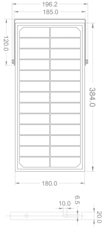
Solar Panel
